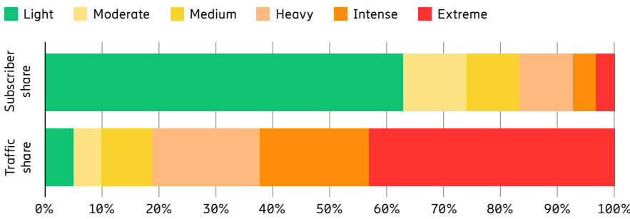
Figure 14: European service provider: Subscriber and traffic volume shares of different subscriber clusters
