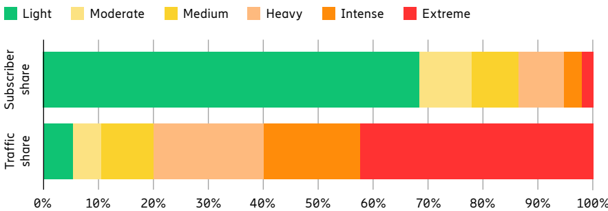
Figure 15: North American service provider: Subscriber and traffic volume shares of different subscriber clusters
