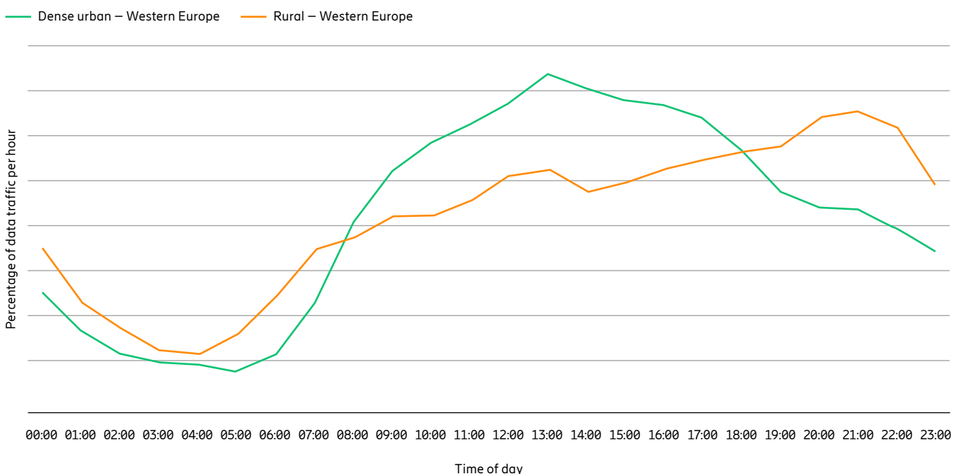
Figure 24: Western Europe hourly traffic over a typical 24 hours
