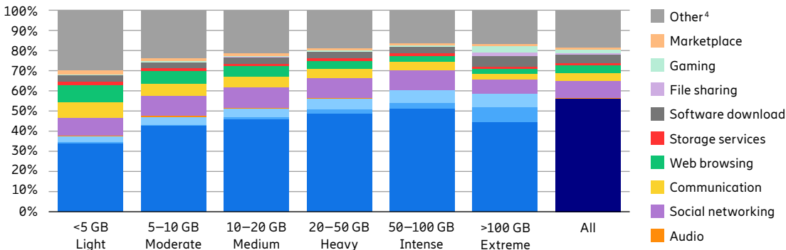
Figure 17: North American service provider: Traffic volume per application type of different subscriber clusters
