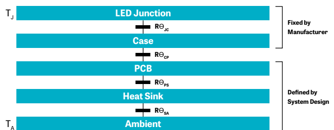
| FIGURE 2: Illustration of thermal model of LED assembly
