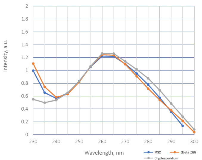
FIGURE 1: Absorption curves for common target microbes.
