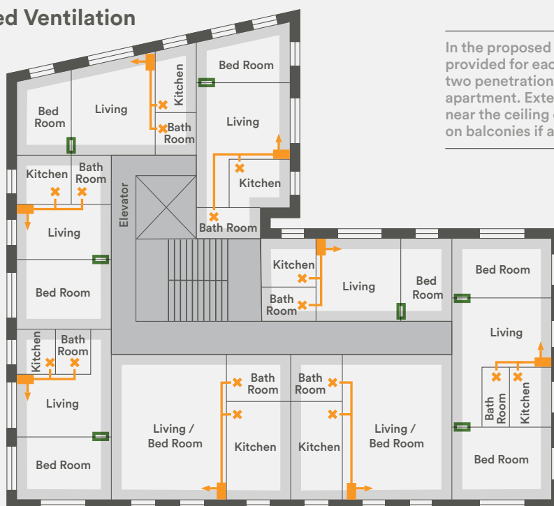
■ Ventilation unit — Ducts x Exhaust ■ Transfer grille o Supply
