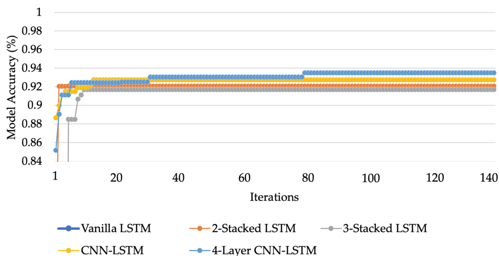
Figure 15. The accuracy of each model after optimization process.
