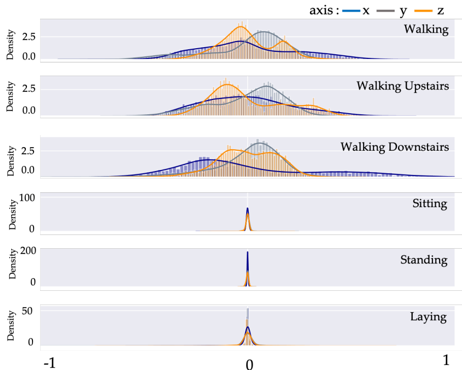
(a) Histograms of the accelerometer data by activity.
