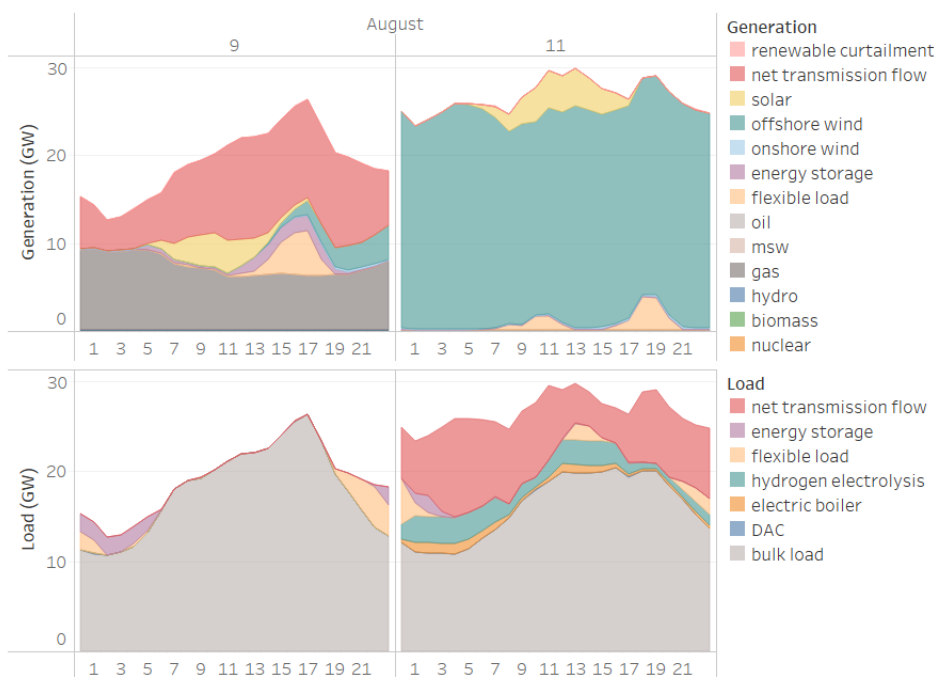
Figure 2.7 Generation and load for a northeastern state in 2050 for (L) a low wind day, and (R) a high wind day.
