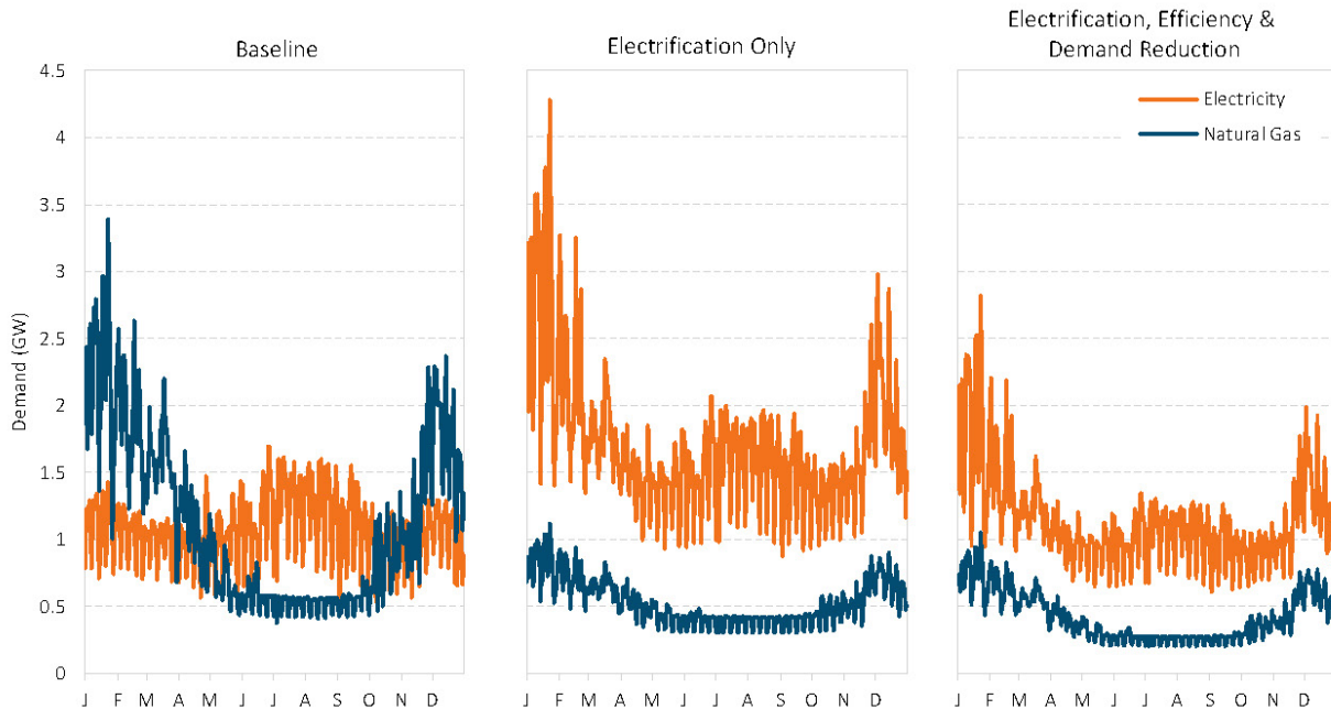
Figure 5.4.2. The impacts of energy efficiency and electrification (Hatchadorian et al., 2019).
