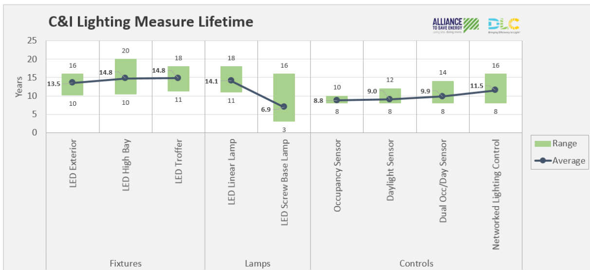
Figure 5: C&I Lighting Measure Lifetimes Based on the TRMs of Twelve EE Programs
