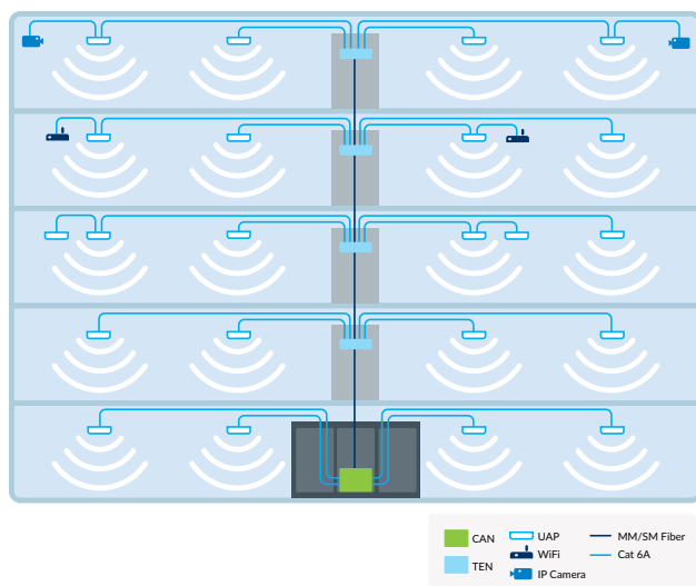
Figure 2: An IT-converged DAS infrastructure uses network cabling instead of expensive coaxial cabling.
